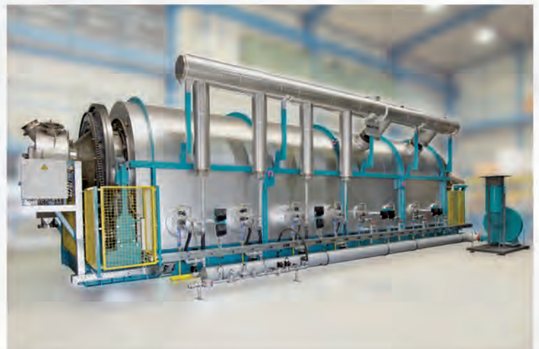
Rotary furnace, indirect gas heated Drehrohröfen, indirekt gasbeheizt
